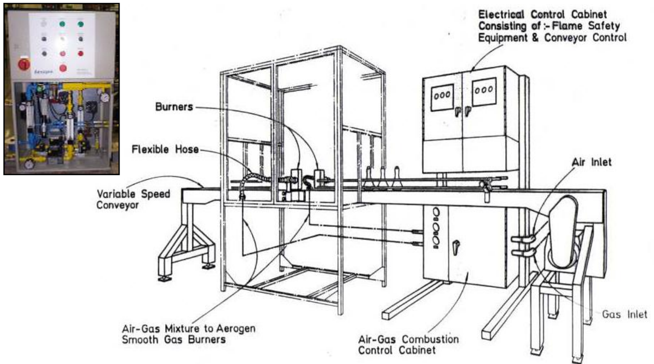
PRETREATMENT SYSTEM FOR P/E CONTAINERS PRIOR TO LABELLING
