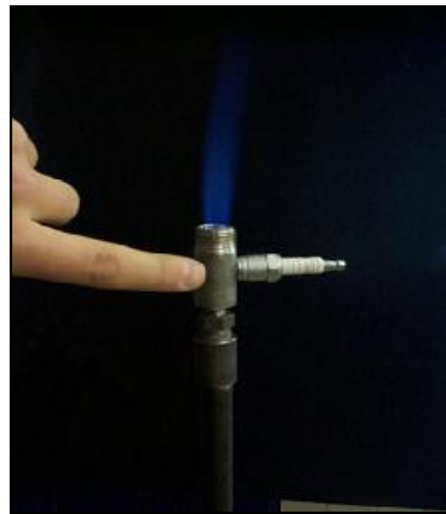
Nozzle Burner Fine Flame Profile
